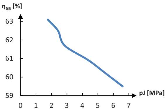
Fig. 9. Relation between the efficiency of combined gas-steam cycle with inter-stage overhear and the partition pressure ( p_J )
