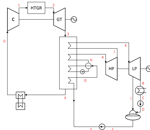
Fig. 4. The combined gas-steam power system fitted with the high-temperature reactor HTGR and inter-stage overheats: C - compressor, HTGR - high-temperature reactor, GT - gas turbine, HP - high-pressure part of steam turbine, LP - low-pressure part of steam turbine
