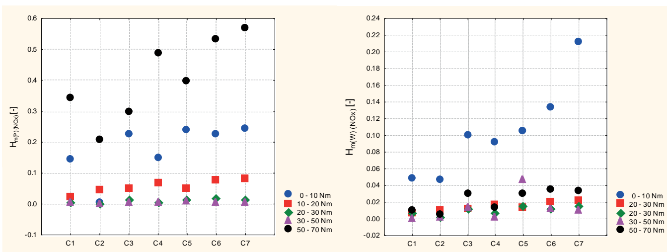
Fig.4. Values of information capacity index H_m for NO_x and transient state: n = 1100 rpm, load change from T_{iq} = 0 Nm to T_{iq} = 70 Nm: P – delayed fuel injection timing, W – advanced fuel injection timing, C1 – C7 – combinations of explanatory variables
