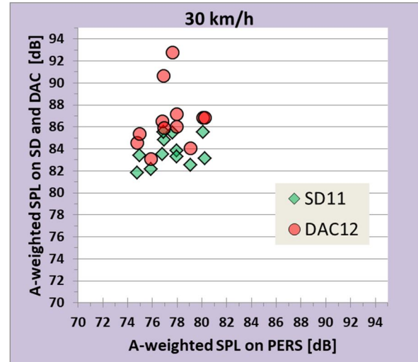
Figure 9. Noise comparison for speed 30 km/h
