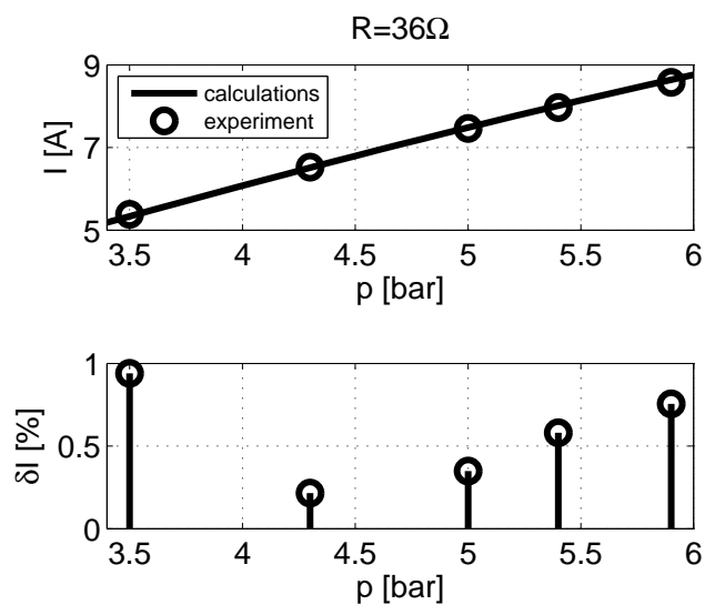
Figure 30: Electric current I of the microturbine set as a function of pressure p at the turbine inlet, for constant load resistance R = 36\ \Omega and relative error \delta I between experiment and calculations
