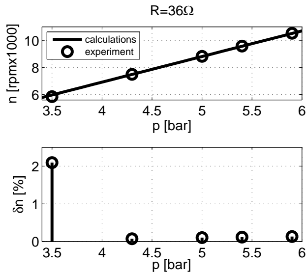
Figure 29: Rotational speed n of the microturbine set as a function of pressure p at the turbine inlet, for constant load resistance R = 36\ \Omega and relative error \delta n between experiment and calculations
