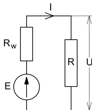
Figure 15: Simplified equivalent circuit diagram of the DC electric part of the microturbine set: E-equivalent DC source potential, R_w -equivalent device resistance, I-electric current, U-voltage, R-resistance of electric energy receiver
