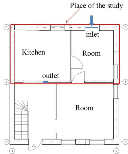
Fig. 2. The residential family detached test house sketch of the first floor.
