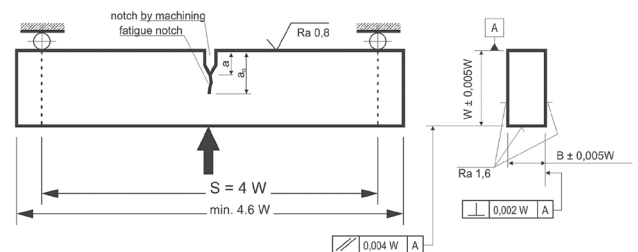
Fig. 2. Bx2B specimen bent at three points for CTOD test, after [10]
