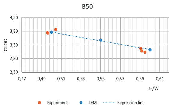
Fig. 11. CTOD as function of a_0/W , based on results of numerical analysis and laboratory tests
