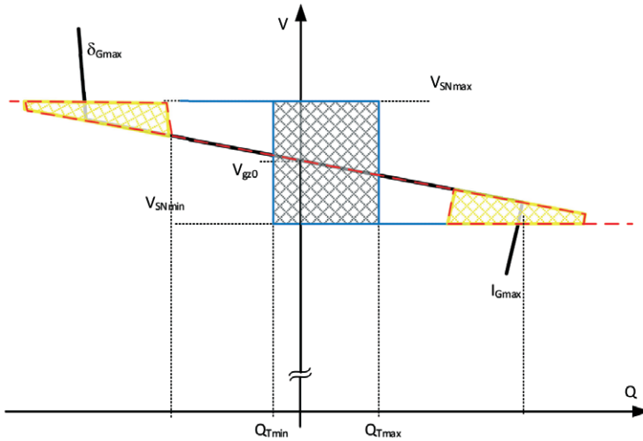
Fig. 9. Resultant characteristic of generators and transformers, where V_{gz0} – voltage setpoint at idle, I_{max} – stator or rotor current limit, \delta_{max} – power angle limit
