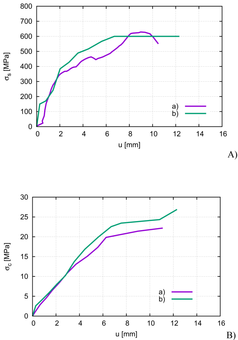
Fig.23: Calculated and measured normal stress \sigma at wall mid-span versus deflection u : A) tensile stress in reinforcement (before failure) at frame beam bottom and B) compressive stress in concrete at frame beam top and (a) experiments and b) FE result within enhanced elasto-plasticity (tensile fracture energy G_f=200 N/m (curve 'a' of Fig.17B), compressive fracture energy G_c=3250 N/m (curve 'b' of Fig.17A), bond-slip with u_0=0.03 mm and characteristic length of micro-structure l_c=5 mm)
