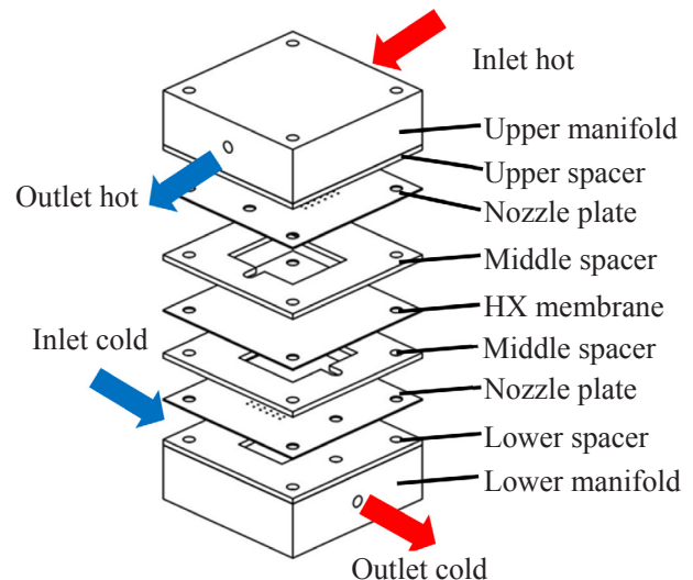
Fig. 2. Schematic of modular microjet heat exchanger.
