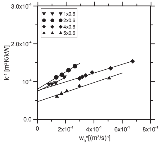
Fig. 6. Sample scheme for calculating the heat transfer coefficient by Wilsons plot method, for various geometries.
