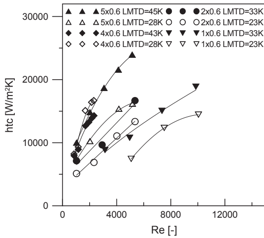
Fig. 7. Experimentally obtained heat transfer coefficient values.
