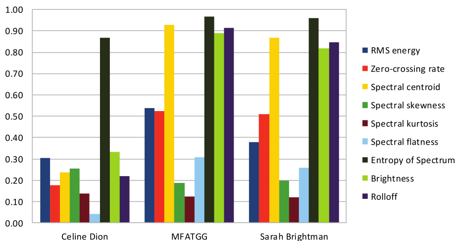
Fig. 13. Original performance different from covers: ( My Heart Will Go On – song by: Celine Dion (pop); covers by: Me First and The Gimme Gimmes (punk rock), Sarah Brightman (musical singer).
