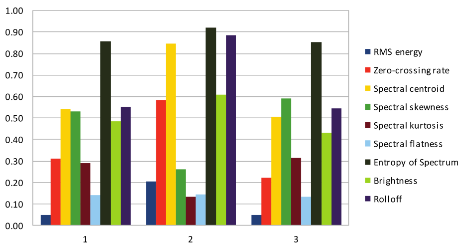
Fig. 14. Green Day's song Minority (1 – beginning, 2 – mid part of the song, 3 – end).
