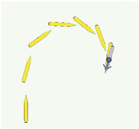
FIGURE 4: Simulation of sample ships turning performed with the use of the full mission bridge simulator at the Faculty of Navigation, Gdynia Maritime University.
