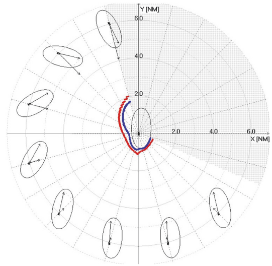
FIGURE 12: Own ship's arenas for a target approaching with a true speed of 18 knots (blue line) or 23 knots (red line) in good visibility. Course alterations of up to 180^\circ to starboard are considered for crossing, course alterations to either side for being overtaken. No speed reduction is assumed.
