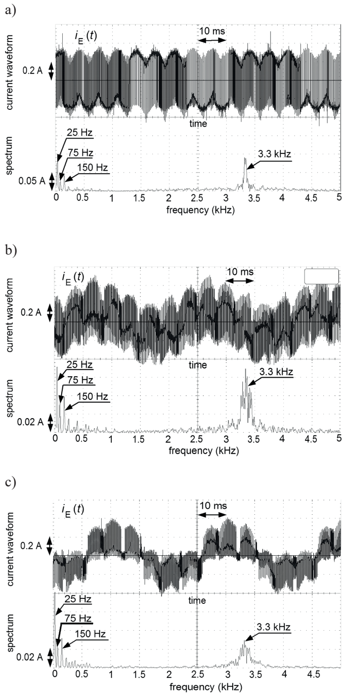
Fig. 9. Earth fault current waveform i_E(t) and its spectrum in circuit with variable-speed drive; motor frequency 25 Hz (50% of the rated motor speed); a) without motor filter, b) with LCF filter, c) with HF filter
