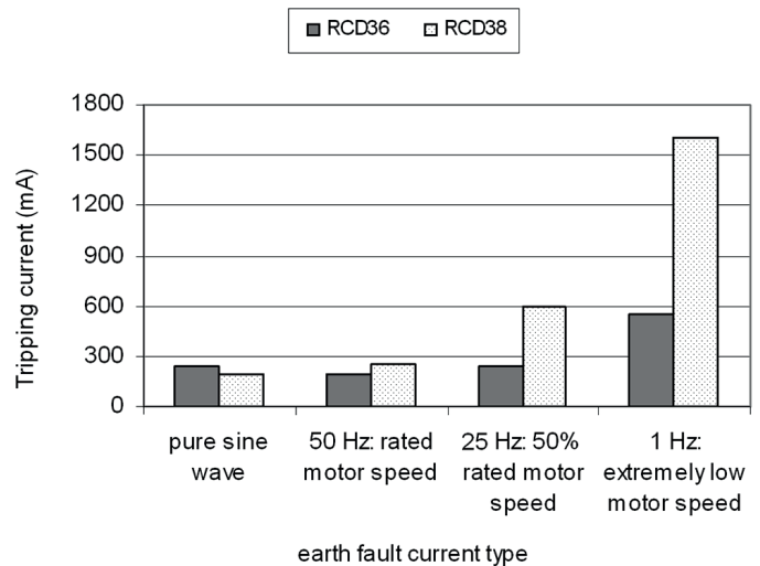
Fig. 21. Tripping current of the selected two RCDs of I_{\Delta n} = 300 mA (RCD36, RCD 38: A-type) for modelled variable-speed drive earth fault currents
