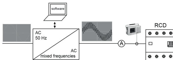
Fig. 15. Simplified diagram of the laboratory stand for testing of tripping current of residual current devices
