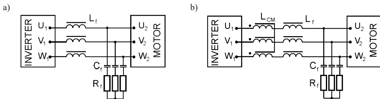
Fig. 2. The structures of the filters used in the investigations: a) LC filter “LCF”: L_f = 9 mH, C_f = 8 \mu F, R_f = 2.2 \Omega , b) hybrid filter “HF”: L_{CM} = 14 mH, L_f = 5.6 mH, C_f = 10 \mu F, R_f = 1 \Omega
