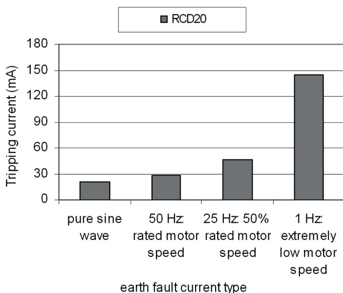
Fig. 22. Tripping current of the selected RCD of I_{\Delta n} = 30 mA, B-type for modelled variable-speed drive earth fault currents
