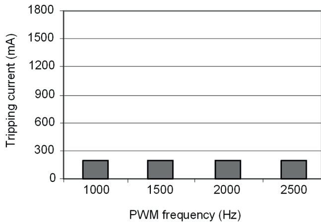
Fig. 24. Tripping current of the proposed RCD of I_{\Delta n} = 300 mA for selected PWM frequency and extremely low motor speed
