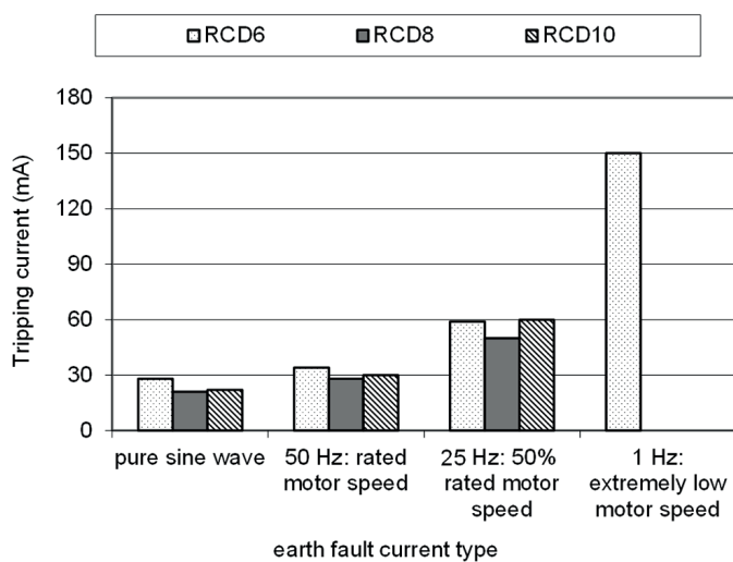
Fig. 17. Tripping current of the selected three RCDs of I_{\Delta n} = 30 mA (RCD6, RCD8, RCD10: AC-type) for modelled variable-speed drive earth fault currents
