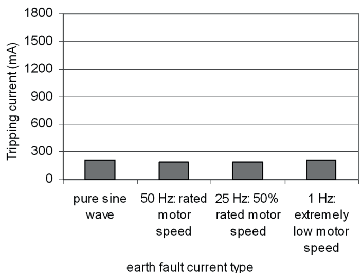
Fig. 23. Tripping current of the proposed RCD of I_{\Delta n} = 300 mA for modelled variable-speed drive earth fault currents
