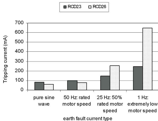
Fig. 19. Tripping current of the selected two RCDs of I_{\Delta n} = 100 mA (RCD23: AC-type; RCD26: A-type) for modelled variable-speed drive earth fault currents
