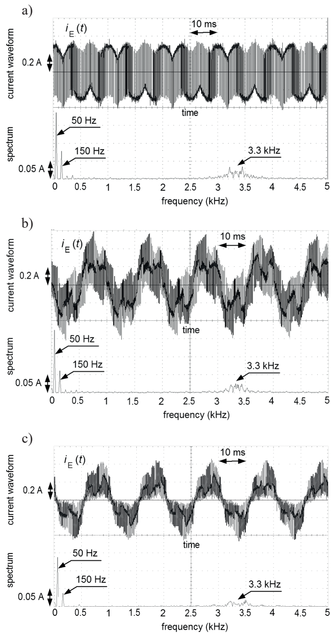
Fig. 8. Earth fault current waveform i_E(t) and its spectrum in circuit with variable-speed drive; motor frequency 50 Hz (rated motor speed); a) without motor filter, b) with LCF filter, c) with HF filter [18]
