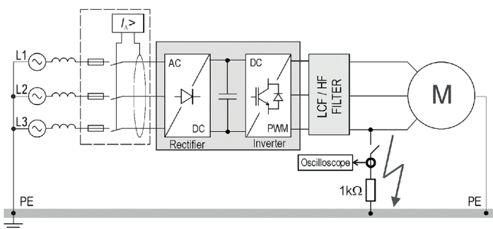
Fig. 3. The structure of the analyzed variable-speed drive circuit [18]
