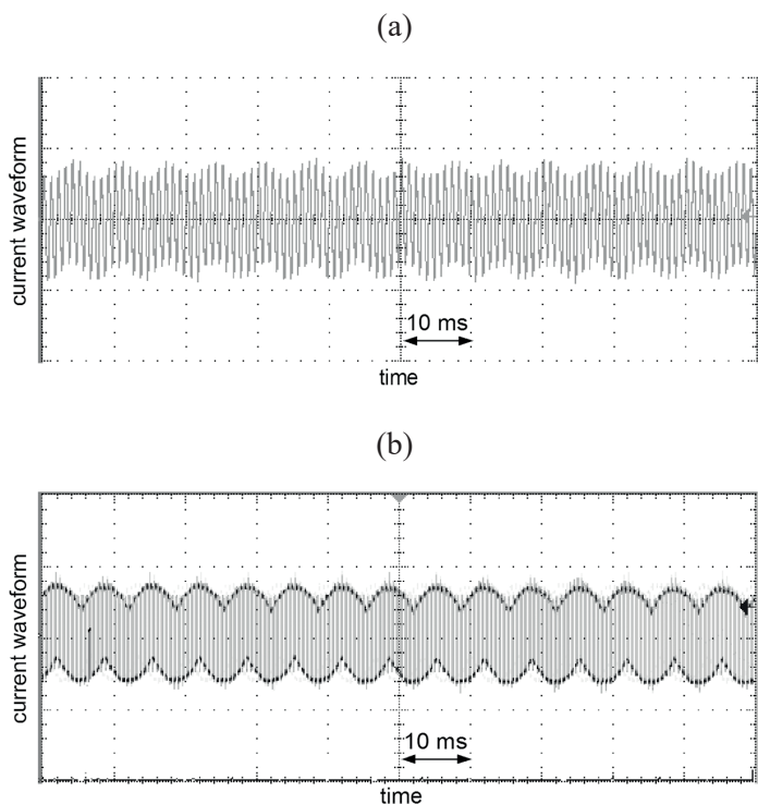
Fig. 16. Earth fault current: a) generated in multi-harmonics generator, PWM frequency 1 kHz; b) from real circuit – PWM frequency 1.67 kHz
