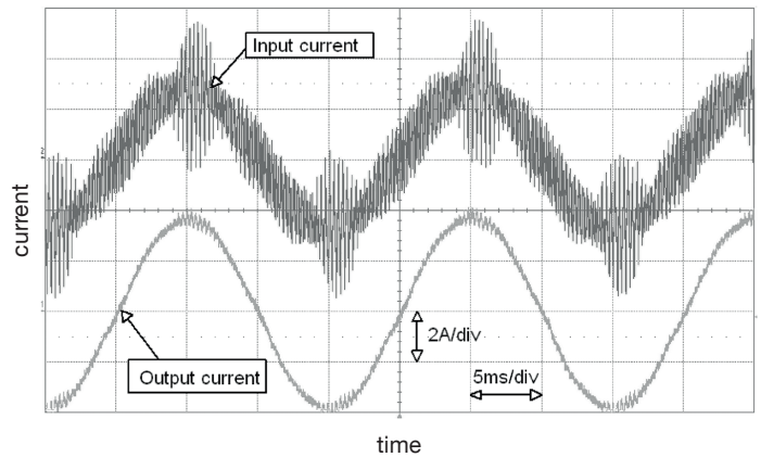
Fig. 5. The waveforms for LCF filter: input current and output current under normal operation – no earth fault, f_{1\text{har}} = 50 \text{ Hz}
