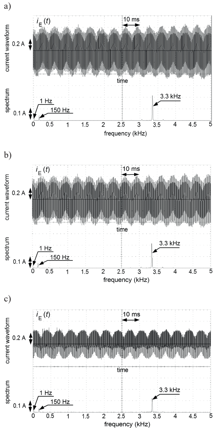
Fig. 10. Earth fault current waveform i_E(t) and its spectrum in circuit with variable-speed drive; motor frequency 1 Hz (extremely low motor speed); a) without motor filter, b) with LCF filter, c) with HF filter [18]
