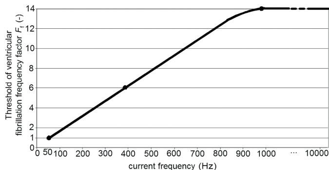
Fig. 12. Frequency factor for the threshold of ventricular fibrillation within the 50 Hz to 10 000 Hz frequency range
