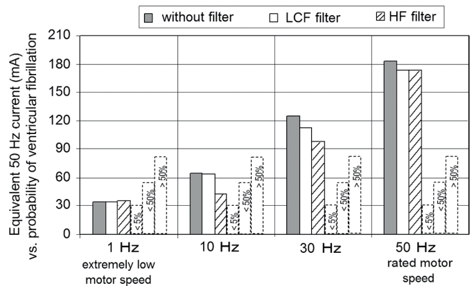
Fig. 13. Example values of equivalent 50 Hz earth fault current vs. probability of ventricular fibrillation
