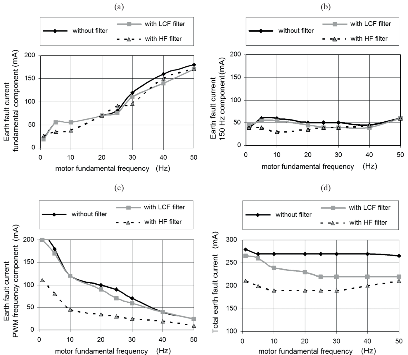
Fig. 11. Content of main components in earth fault current as a function of motor fundamental frequency: a) motor fundamental component, b) 150 Hz, c) PWM frequency, d) total earth fault current
