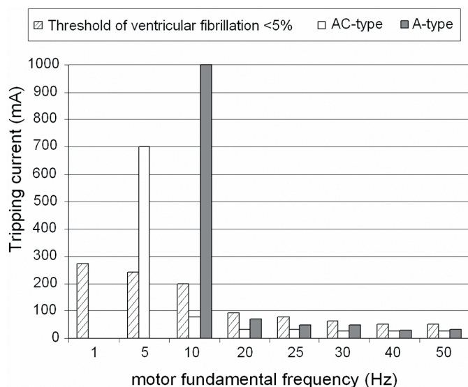
Fig. 14. Tripping current of the selected two RCDs (AC-type and A-type) versus threshold of ventricular fibrillation; no motor filter in the circuit
