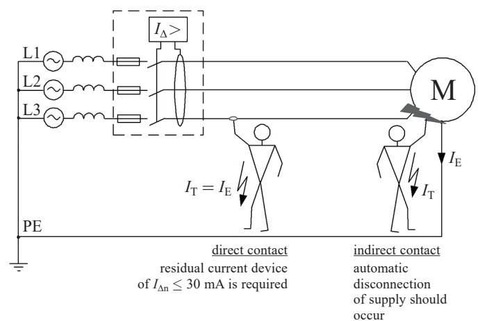
Fig. 1. Direct and indirect contact in a circuit, and requirements to achieve safety; ( I_{\Delta} > ) – residual current device, I_E – earth fault current, I_T – touch current
