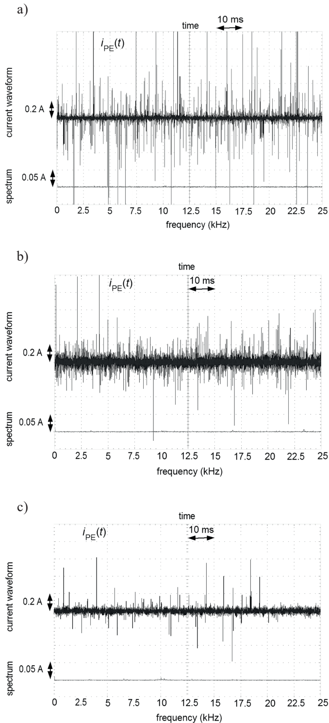
Fig. 7. Current in PE conductor under normal operating conditions i_{PE}(t) and its spectrum in circuit with variable-speed drive; rated motor speed (50 Hz); a) without motor filter, b) with LCF filter, c) with HF filter [18]
