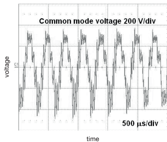
Fig. 6. The waveform of common mode voltage for LCF filter under normal operation – no earth fault, f_{1\text{har}} = 25 \text{ Hz} [18]
