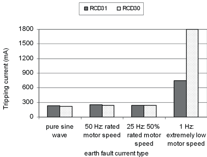
Fig. 20. Tripping current of the selected two RCDs of I_{\Delta n} = 300 mA (RCD30, RCD 31: AC-type) for modelled variable-speed drive earth fault currents
