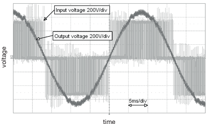
Fig. 4. The waveforms for LCF filter: line-to-line input and output voltage under normal operation – no earth fault, f_{1\text{har}} = 30 \text{ Hz}
