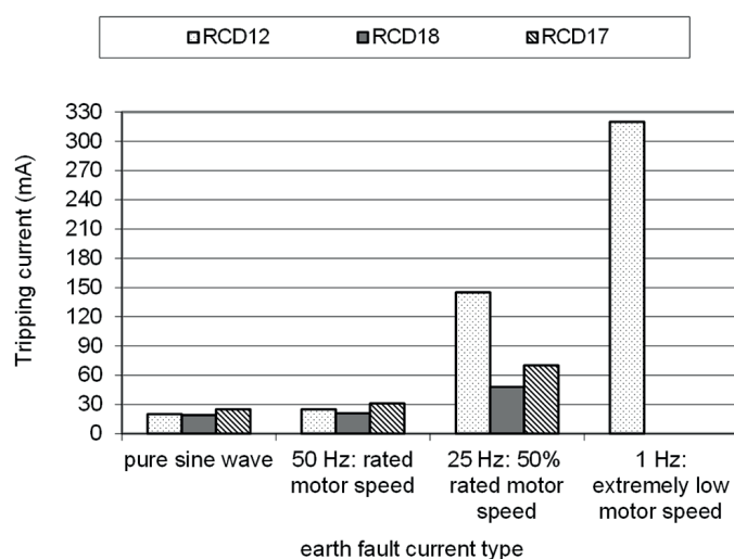
Fig. 18. Tripping current of the selected three RCDs of I_{\Delta n} = 30 mA (RCD12, RCD17, RCD18: A-type) for modelled variable-speed drive earth fault currents
