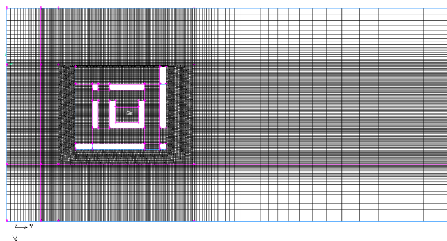
Fig. 5. The mesh in XY plane
