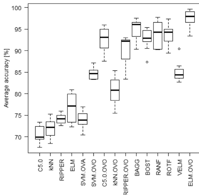
Fig. 2. Boxplot of average accuracy (%) metric obtained examined classifiers used in the proposed intelligent marine engine fault detection system.
