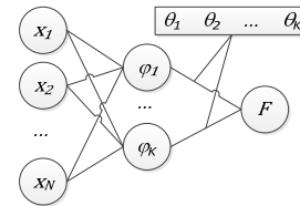
Fig. 2. Simplified scheme of RBF network structure
