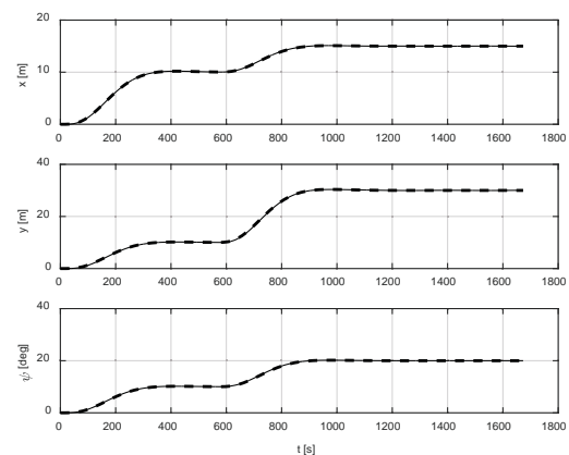
Fig. 4. Set (--) and real (-) time-histories of ship position and heading
