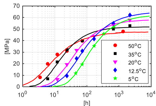
Fig. 2. Mortar compressive strength [22]
