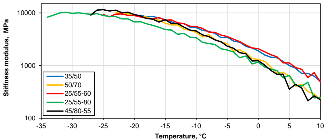
342 Fig. 10. Back-calculated values of stiffness moduli for different bitumen types.
