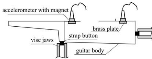
Fig. 6. Strap buttons fixed between vise jaws and accelerometers fastening using brass plates and embedded magnets.
