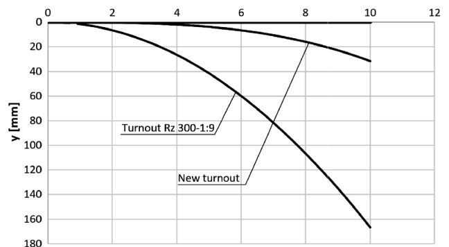
Fig. 10. Outline of the curved switch blade and closure rail position in an example turnout with softened curvature of the diverging track and a traditional turnout (in a non-comparative scale) [own elaboration]
