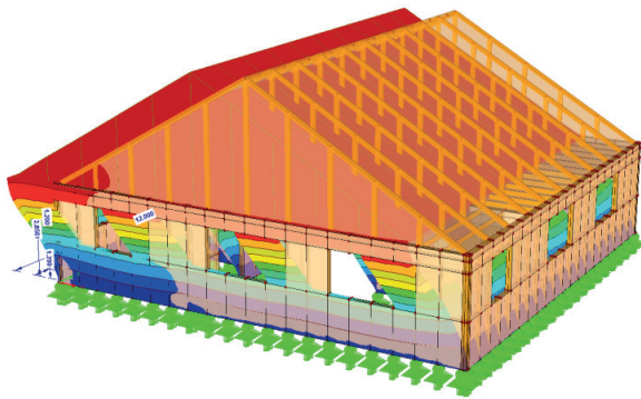
Fig. 3 1 st eigenform for the building with mineral wool ( f_1 = 1.890 Hz)
