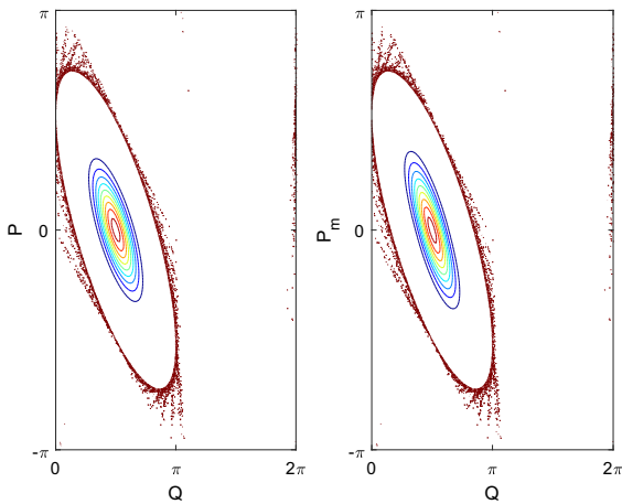
Fig. 5 Absolute value of Wigner functions for n = 0 (left side) and n = 4000 (right side). Dots represent the sticking area of classical AM, P = P_m \bmod 2\pi
