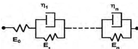
Fig. 1 Generalized Kelvin-Voigt model adopted with an additional Hooke element (GK-H)
