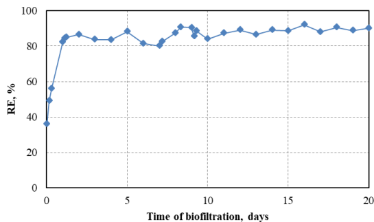
Fig. 2. Performance of a biotrickling filter packed with a mixture of peat and perlite.
