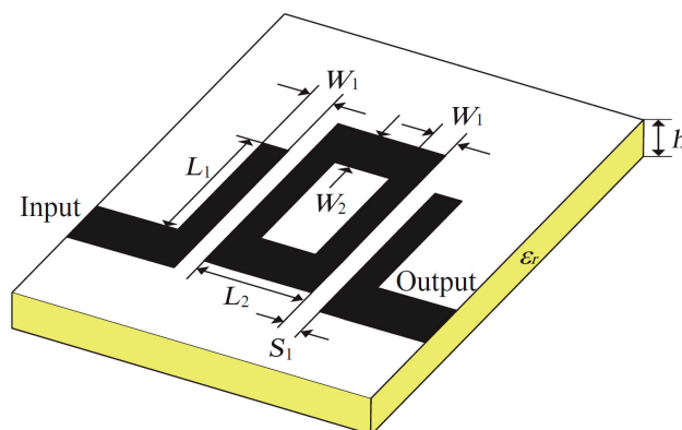
Figure 3. Second-order ring resonator bandpass microstrip filter: geometry [12,17].
