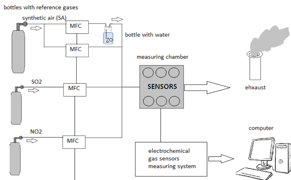
Fig. 1. Structure of the measuring stand
