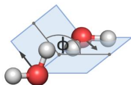
Fig. 2 Definition of a \phi angle between two water molecules connected by a hydrogen bond (the bisectors of the H-O-H angles for both water molecules are indicated by arrows)
