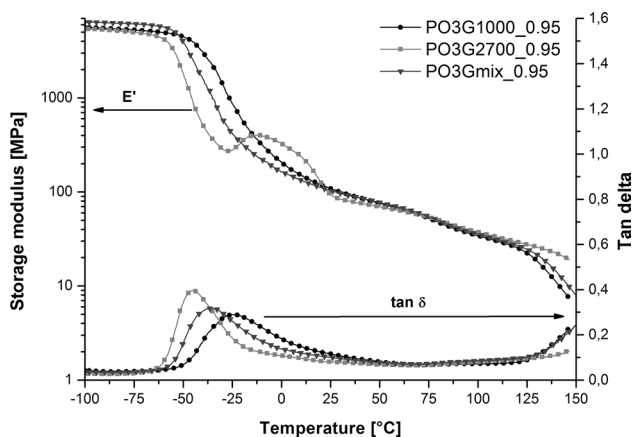
Fig. 7 DMTA thermograms presenting the dependence of the storage modulus and tan δ as a function of temperature for TPUs obtained with different prepolymers
