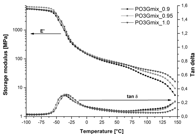
Fig. 6 DMTA thermograms presenting the dependence of the storage modulus and tan δ as a function of temperature for TPUs obtained from the mixture of prepolymers
