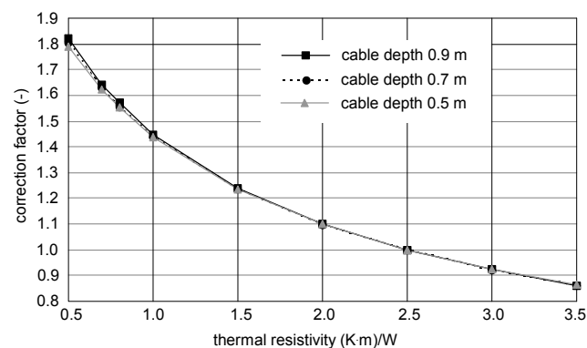
Fig.2. Correction factors of the current-carrying capacity calculated according to IEC 60287 [12, 13], for a cable YKY 1×240 mm 2 (copper conductor, PVC insulation and sheath) directly buried in the ground, for various thermal resistivities of the soil and cable depth. Reference thermal resistivity of the soil: 2.5 (K·m)/W
