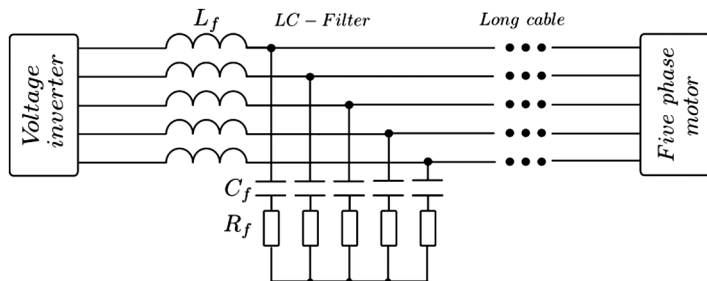
Fig. 2. LC filter structure in a five-phase drive system.
