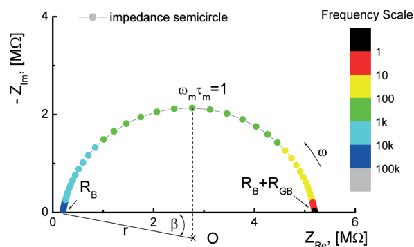
Fig. 3. Impedance plane plot for a depressed circular arc; \beta -depression angle. Meaning of all the parameters is illustrated
