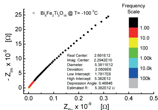
Fig. 5. Impedance diagrams in the complex Z''-Z' plane measured for \text{Bi}_6\text{Fe}_2\text{Ti}_3\text{O}_{18} ceramics at temperature T=0^\circ\text{C} (a), T=-100^\circ\text{C} (b); isotropic (a) and free scale (b) was used for data presentation
