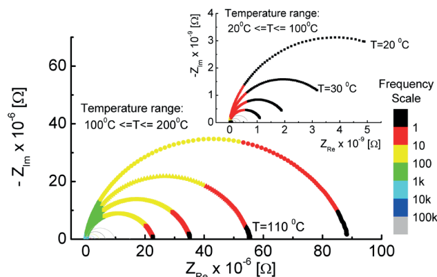
Fig. 2. Comparison of impedance spectra plotted in Z''-Z' plane for \Delta T = 20 - 200^\circ\text{C}
