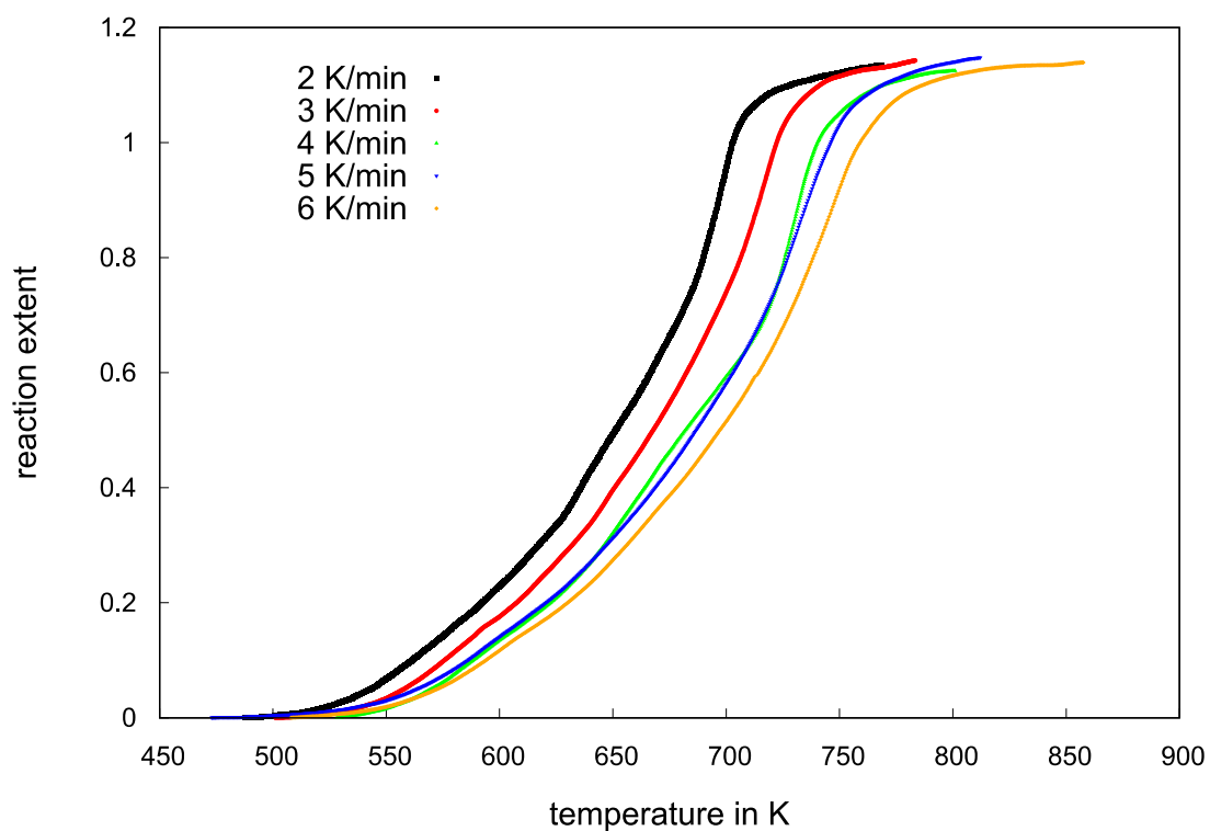
Fig. S23. Dependence of reaction extent on temperature for \text{Bi}_2\text{O}_3+\text{TeO}_2 reduction
