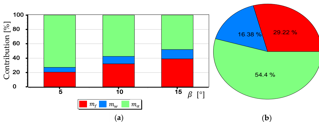
Figure 30. Percentage contribution for DIJ FC550RAW camera: (a) Calculated for \beta equals 5°, 10° and 15°; (b) Calculated as a mean value.
