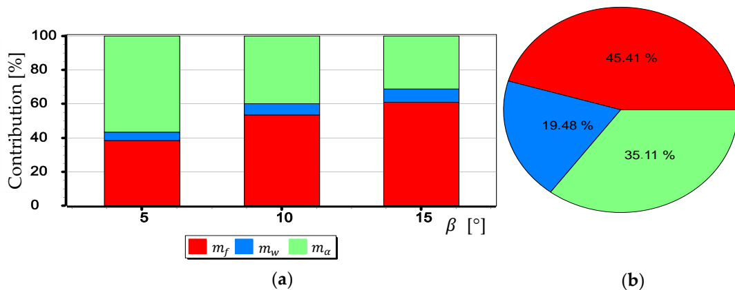
Figure 28. Percentage contribution for DIJ FC220 camera: (a) Calculated for \beta equals 5^\circ, 10^\circ and 15^\circ ; (b) Calculated as a mean value.
