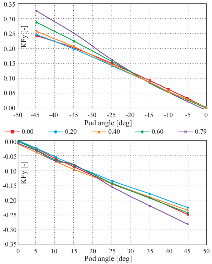
Fig. 10. Transverse force coefficient vs. deflection angle.
