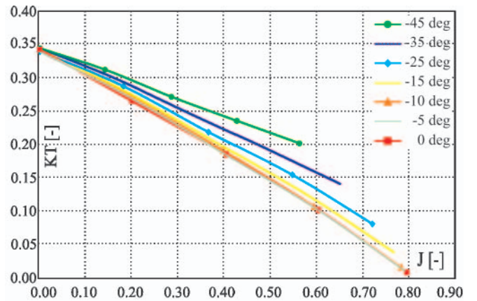
Fig. 14. Transverse force coefficient vs. advance coefficient.
