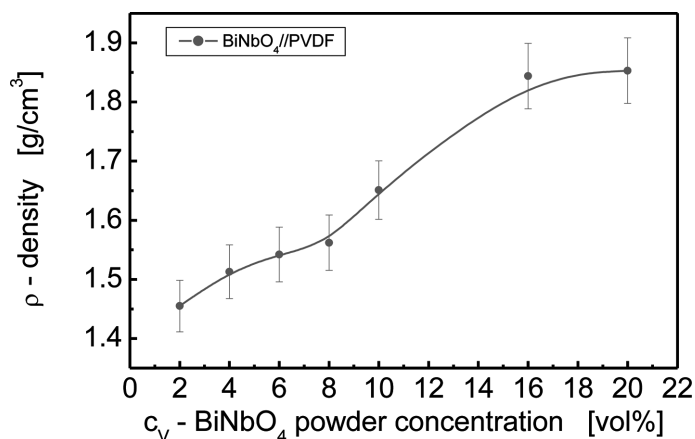
Fig. 3. Apparent density of \text{BiNbO}_4 //PVDF composites
