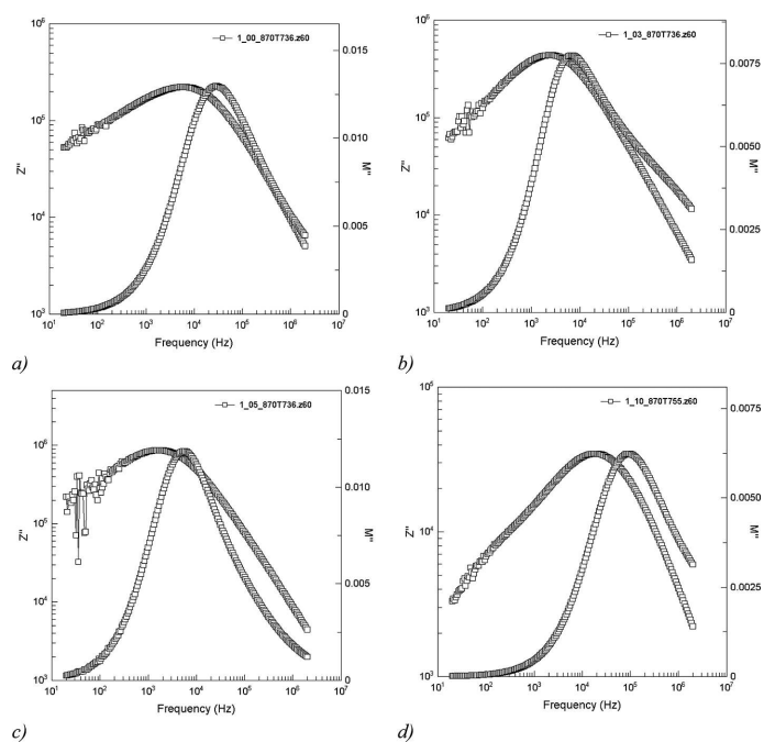
Fig. 4. Combined plots of Z''(\nu) and M''(\nu) spectra showing lack of coincidence of maxima on the frequency scale at T \approx 463^\circ\text{C} for \text{BiNbO}_4 ceramics: a) – 0 mol%; b) – 3 mol%; c) – 5 mol% and d) – 10 mol% of \text{Bi}_2\text{O}_3 excess
