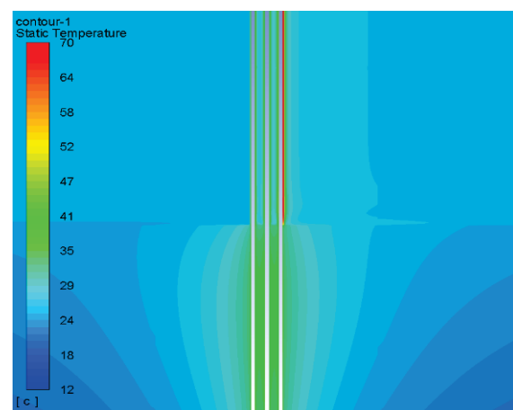
Figure 3 Temperature distribution around the surface of power cables – with solar radiation, wind from left to right v_{\text{wind}} = 1\text{ m/s} , symmetric load: I_{zL1} = I_{zL2} = I_{zL3} = 122,3\text{ A}
