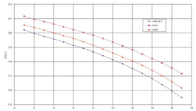
Fig. 5. Compensator location impact on voltage variability at busbars of a) 220/110 kV substation, b) 400/110 kV substation [19]
