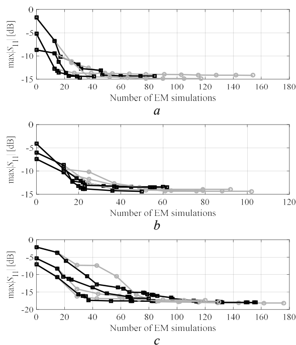
Fig. 5. Convergence plots for selected algorithm runs: reference algorithm (gray) and the proposed algorithm with N_{iter} = 5 and E = 1 (black).
