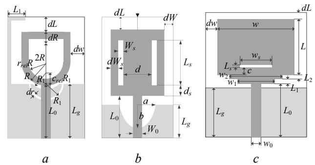
Fig. 1. Antenna structures used for verification of the proposed algorithm. Ground plane marked using light gray shade.
