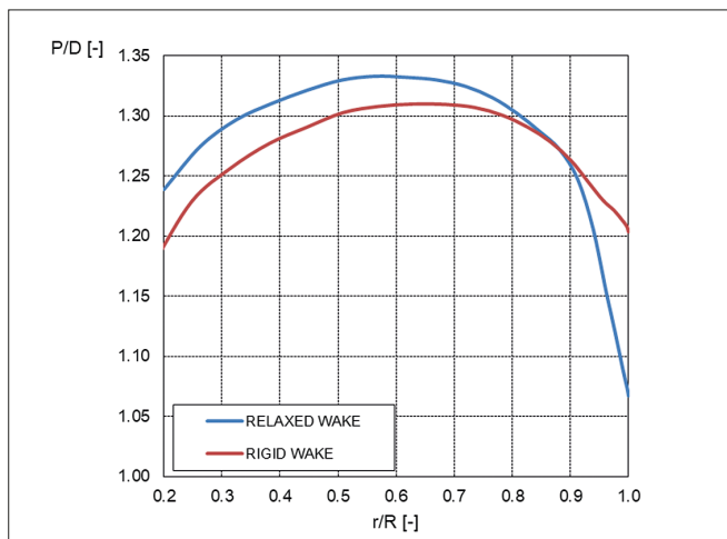
Fig. 4. Influence of vortex wake on blade's pitch
