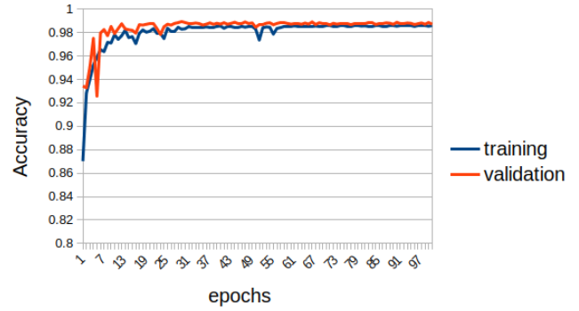
Fig. 4. Training and validation accuracy analysis over 100 epochs
