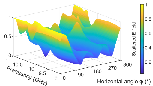
Fig. 3. The plots of the normalized scattered far-field as a function of frequency and angle \varphi .
