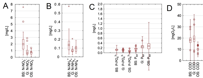
Figure 2 Concentrations of COD, nitrogen and phosphorus species in the analysed streams. (A) Concentration of NO 3 - , (B) concentration of NH 4 + , (C) concentration of P-PO 4 3- and P tot , (D) concentration of COD. BS, the Bładzickowski Stream; G, the Gizdepka; OS, the Oliwski Stream.
