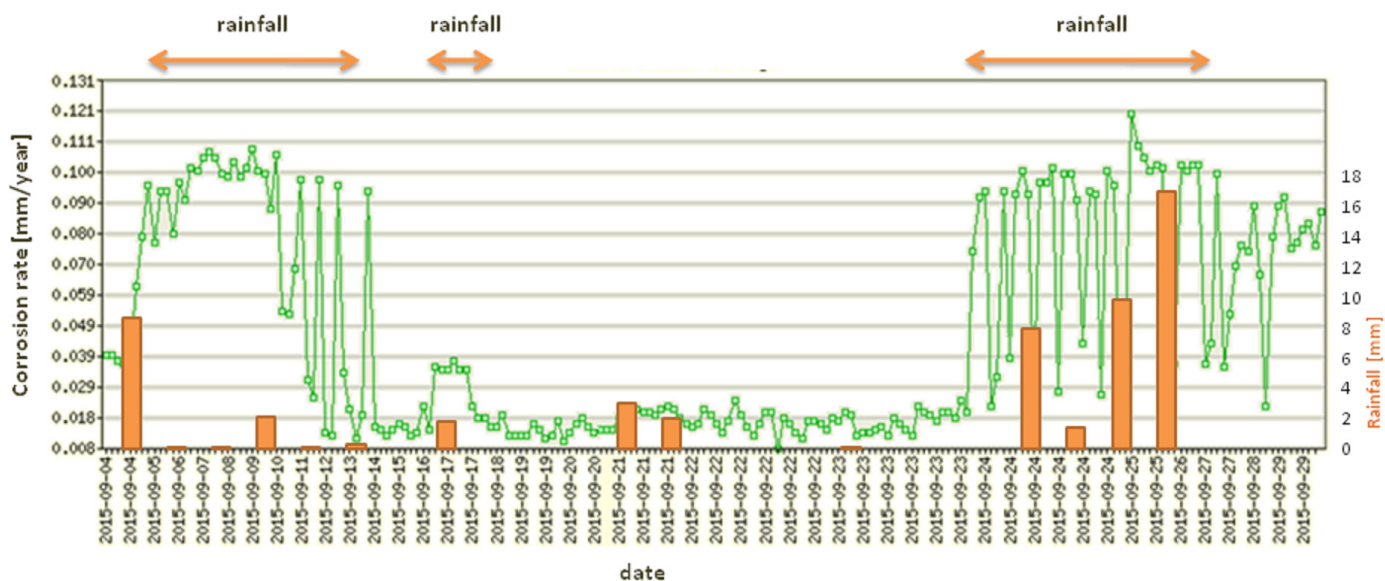
Fig. 8. Influence of rain on the corrosion rate in Kopiec location (orange bar – rainfall, green line corrosion rate)
