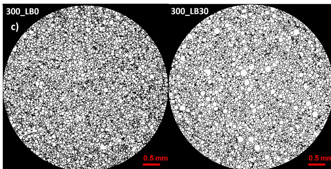
Figure 2. 2D images of PUR-PIR foams: (a) I_{ISO} = 200 , (b) I_{ISO} = 250 , (c) I_{ISO} = 300 .
