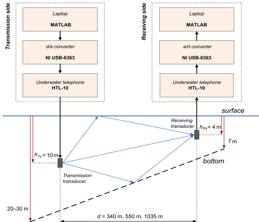
Fig. 3. Measuring system.
