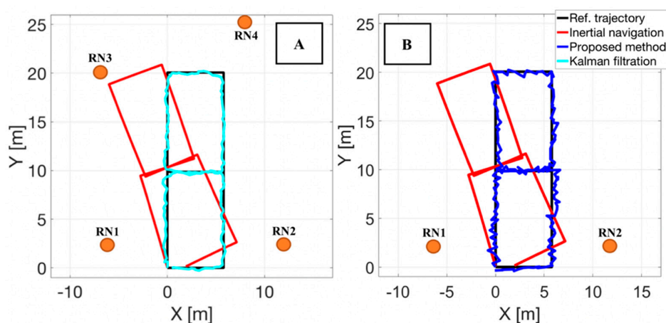
Figure 6. Results of a person tracking in a simulated hybrid localization system when a known approach based on fusion Kalman filtration (A) and the proposed method (B) was used.
