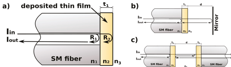
Figure 1. Different designs of fiber-optic Fabry-Pérot interferometers: (a) Interferometer with thin film sensing cavity; (b) and (c) Interferometers with extrinsic sensing cavity operating in reflective and transmission modes, respectively. n_1 —refractive index of the fiber; n_2 —refractive index of the film; n_3 —refractive index of the medium in the cavity; t_1, t_2 —thickness of the thin films; d —length of the cavity.
