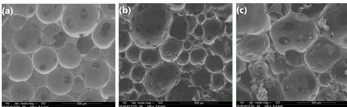
Fig. 6. SEM images of (a) reference PU foam, (b) foam containing 30 pbw (parts by weight) of unmodified WTR and (c) foam containing 30 pbw of devulcanized WTR (Images from (Piszczyk et al., 2015b)).
