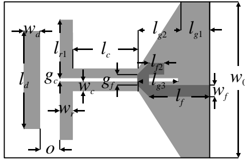
Fig. 3. Quasi-Yagi antenna with a director fed through a microstrip-to-coplanar stripline transition balun. Feed line marked using dark grey shade.
