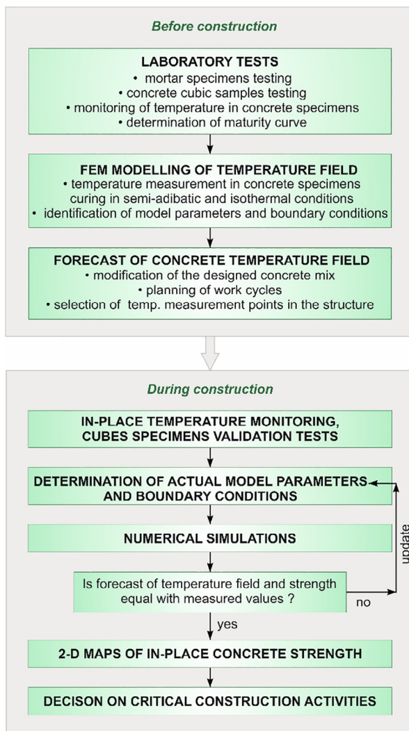
Fig. 2. The research algorithm.
