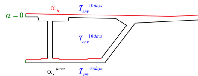
Fig. 8. Boundary conditions.
