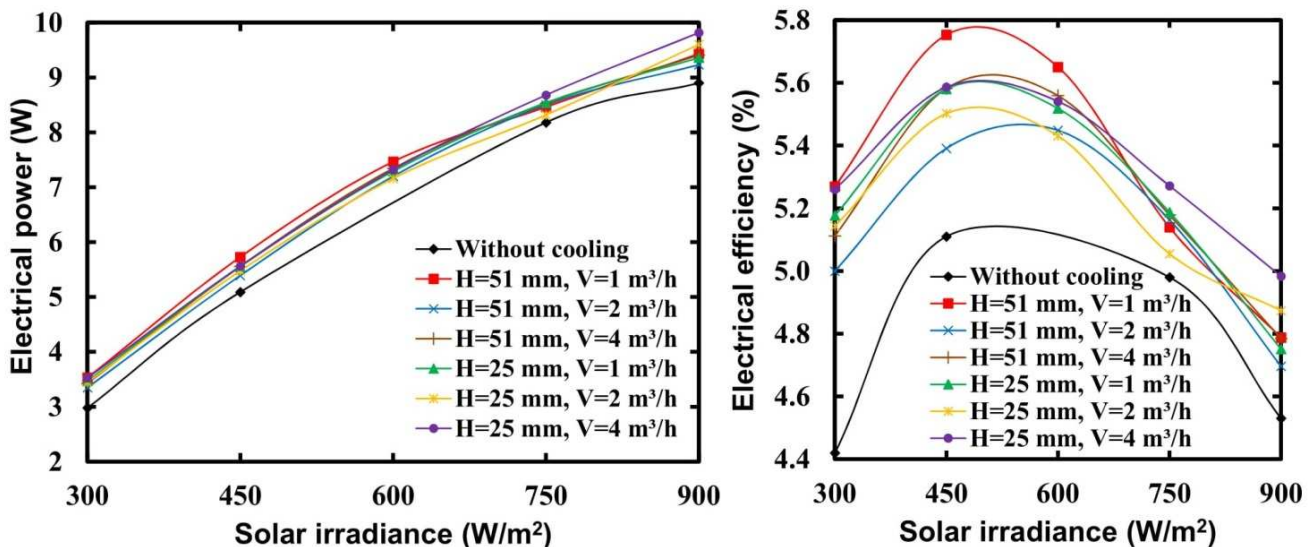
Fig. 5. Electrical characteristics of the PV roof tile as a function of the solar irradiance: (a) generated electrical power, (b) electrical efficiency.
